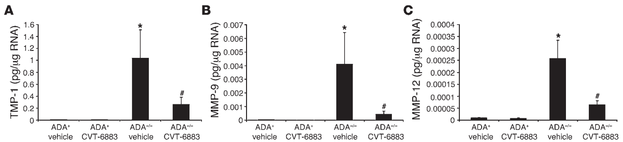
Figure 6 CVT-6883 treatment inhibits the expression of genes associated with alveolar airway destruction. Transcript levels of TIMP-1 (A), MMP-9 (B), and MMP-12 (C) were measured in whole-lung RNA extracts from postnatal day 38 mice using quantitative RT-PCR. Data are mean pg transcript/ \mu g RNA \pm SEM. * P \leq 0.05 versus vehicle-treated ADA^+ mice; # P \leq 0.05 versus vehicle-treated ADA^{-/-} mice. n = 4 ( ADA^+ ), 8 ( ADA^{-/-} ).
