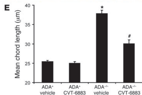
Figure 5 CVT-6883 treatment inhibits alveolar airway enlargement in ADA-/- mice. Lungs from postnatal day 38 mice were infused with fixative under constant pressure (25 cm H 2 O) and processed for H&E staining. (A) Lung from an ADA+ mouse treated with vehicle. (B) Lung from an ADA+ mouse treated with CVT-6883. (C) Lung from an ADA-/- mouse treated with vehicle. (D) Lung from an ADA-/- mouse treated with CVT-6883. Images are representative of 8 animals from each group. Scale bars: 100 μm. (E) Alveolar airspace size was calculated using Image-Pro analysis software; data are mean chord length ± SEM. *P ≤ 0.05 versus vehicle-treated ADA+ mice; #P ≤ 0.05 versus vehicle-treated ADA-/- mice. n = 5 per group.
